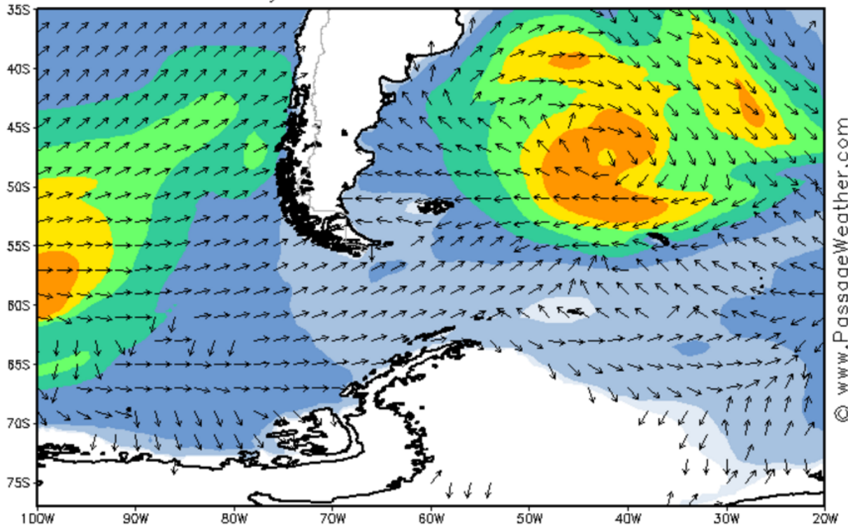
Wave Height (m) and Direction WW3 000 Hour Analysis
