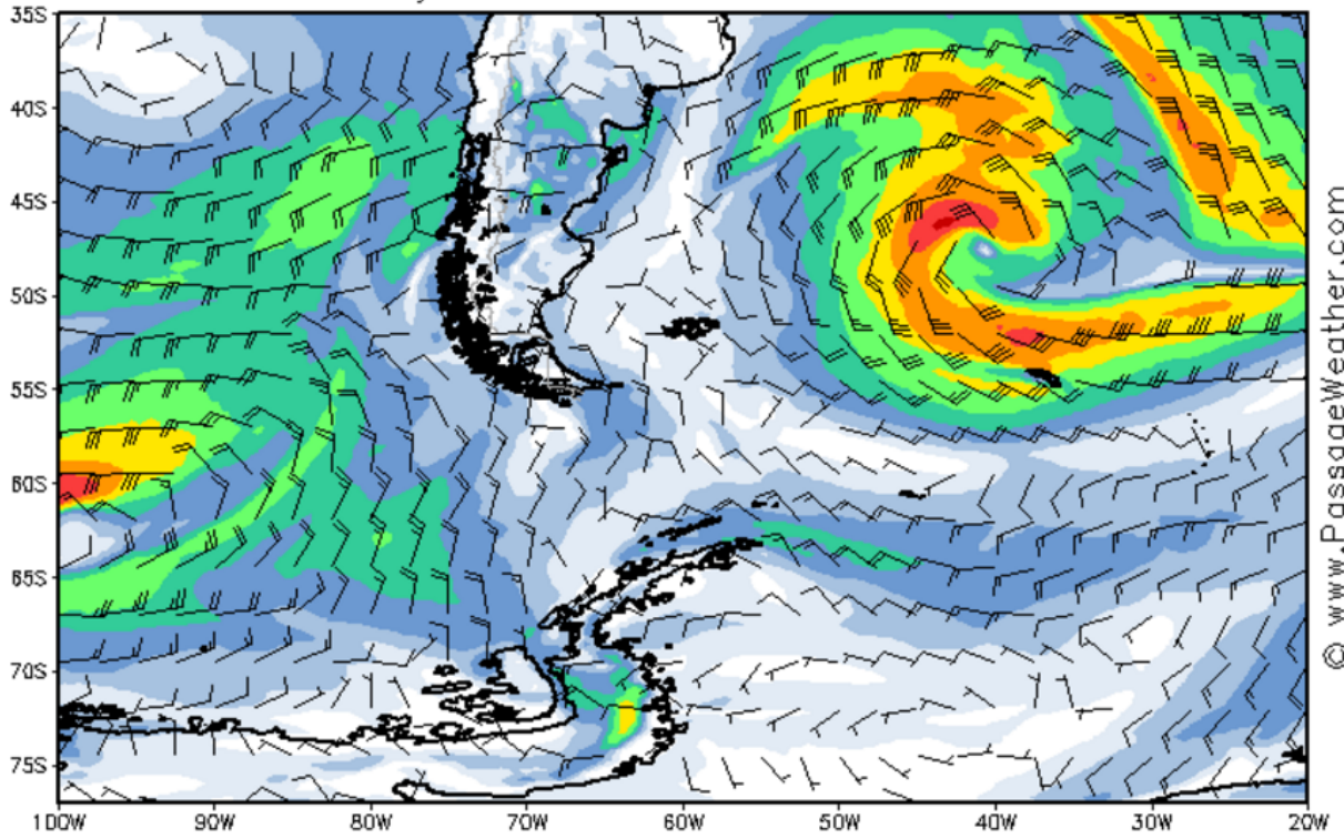
Surface Wind (knots) GFS 000 Hour Analysis
